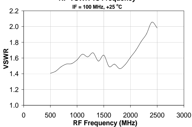
RF VSWR vs Frequency
